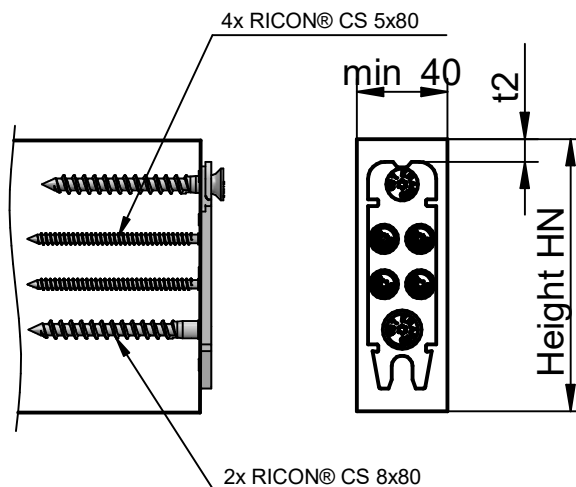
screw pattern for secondary beam
